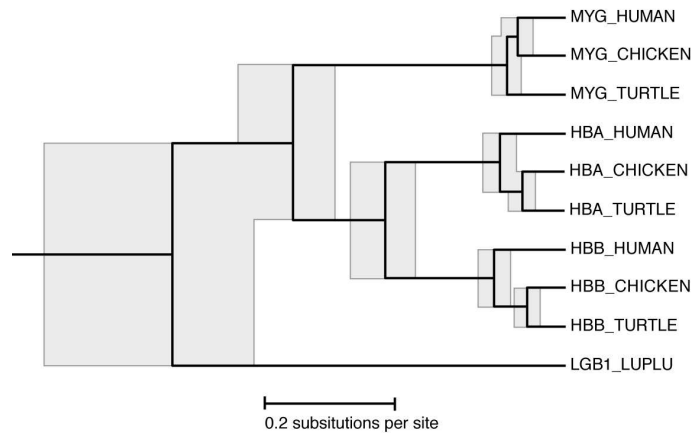
Fig. 1.13. The maximum posterior tree (black) relating the ten globins of Fig. 1.12, and 95% confidence intervals of the node heights (grey boxes). Most of the tree's topology is well determined, with the exception of the myoglobin subtree. Note that this relatively unresolved topology differs from the more well-defined topologies down the alpha and beta hemoglobin branches, that both conform to the accepted phylogeny of human, chicken and turtle.
